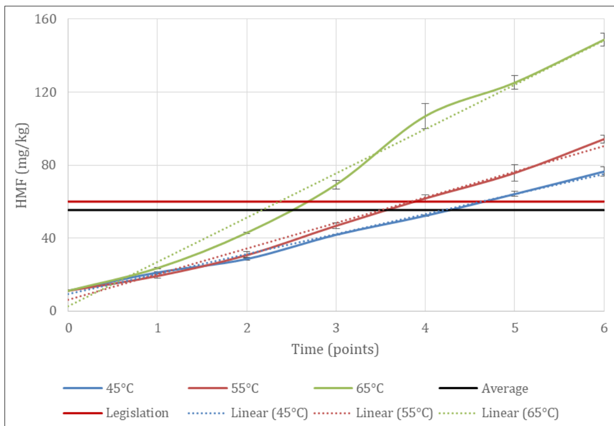
Figure 1 ▼ HMF content over time. Source: research data
