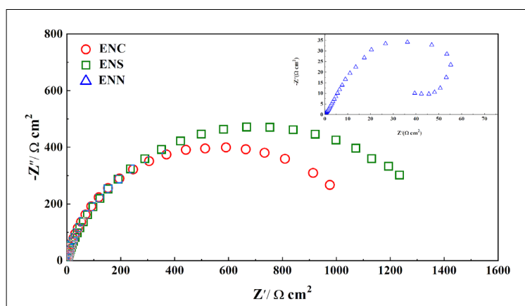
Figure 3 ► Nyquist plots for ENC (red), ENS (green), and ENN (blue) obtained in 3% NaCl solution at 25 °C. Source: research data
