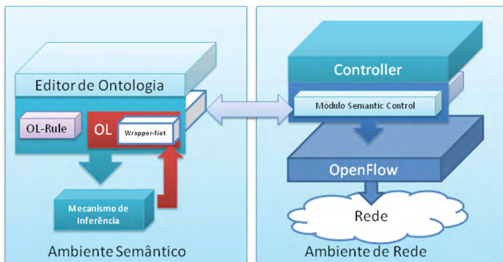
Figura 2. Framework ProNet com o módulo Semantic Control .
